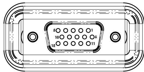
DB15 Female
