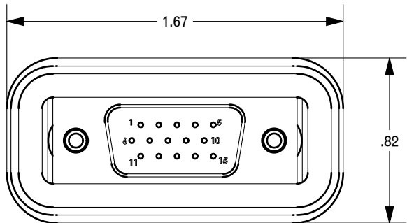
DB15 Male
