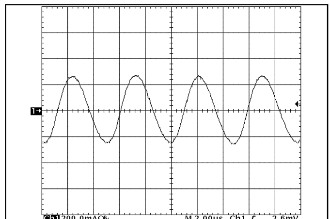
Figure 24: Input Terminal Ripple Current, 3.3V & 5.0V outputs at 50% rated output current and nominal input voltage with 10µH source impedance and 100µF electrolytic capacitor (200 mA/div). (see Fig. 23)
