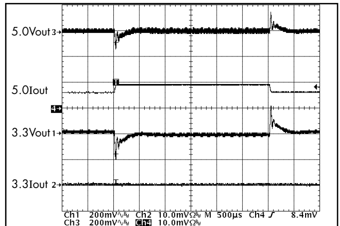
Figure 22: Output voltage response to step-change in Iout2 (50%-75%-50% of Imax; di/dt = 0.1A/\mu s ). Load cap: 15µF, 300 mΩ ESR tantalum cap & 1µF ceramic cap.. Vout (200mV/div), Iout (10A/div). Ch1:Vout1; Ch2:Iout1; Ch3:Vout2; Ch4:Iout2
