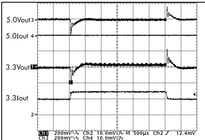
Figure 21: Output voltage response to step-change in Iout1 (50%-75%-50% of Imax; di/dt = 0.1A/\mu s ). Load cap: 15µF, 300 mΩ ESR tantalum cap & 1µF ceramic cap. Vout (200mV/div), Iout (10A/div). Ch1:Vout1; Ch2:Iout1; Ch3:Vout2; Ch4:Iout2
