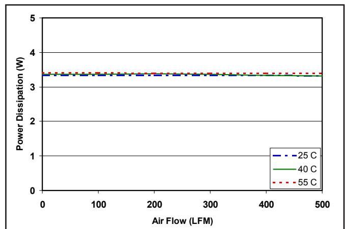
Figure 6: Power dissipation at 100% load and 50/50 voltage split (6.1A load on 3.3V and 4A load on 5.0V) versus air flow rate for ambient air temperatures of 25°C, 40°C, and 55°C. (nominal input voltage).
