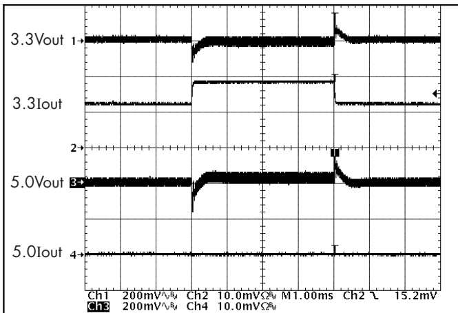
Figure 21: Output voltage response to step-change in Iout1 (50%-75%-50% of Imax; di/dt = 0.1A/\mu s ). Load cap: 15 \mu F , 300 m \Omega ESR tantalum cap & 1 \mu F ceramic cap. Vout (200mV/div), Iout (5A/div). Ch1: Vout1; Ch2 Iout1; Ch 3: Vout2; Ch 4 Iout2
