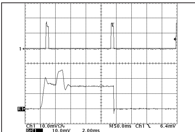
Figure 29: Load current for 3.3V output (10A/div) as a function of time when the converter attempts to turn on into a 10\ \text{m}\Omega short circuit. Bottom trace is an expansion of the on-time portion of the top trace.
