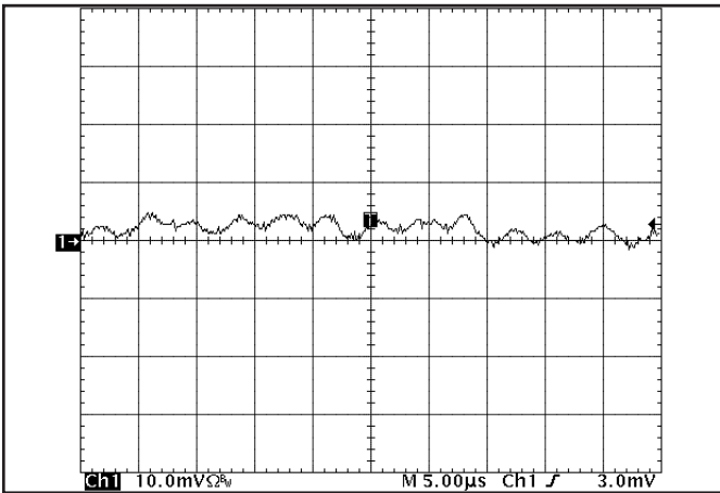
Figure 19: Input Reflected Ripple Current, i_s , through a 10\ \mu\text{H} source inductor at nominal input voltage and rated load current ( 5\ \text{mA}/\text{div} ). 2.5\text{V} and 3.3\text{V} outputs at full rated load current. (see Fig. 17)
