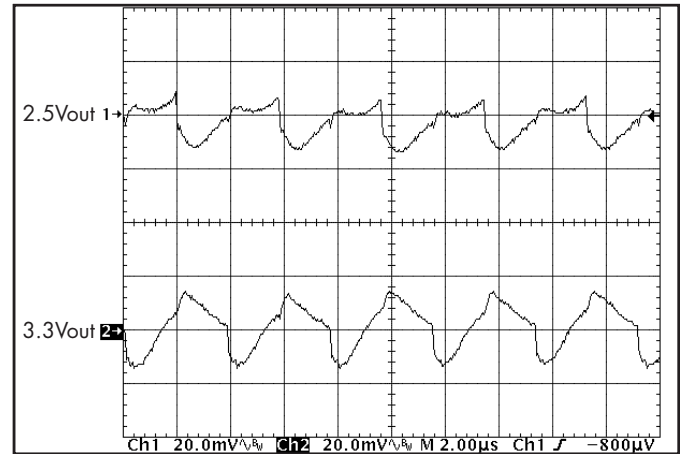
Figure 20: Output Voltage Ripple at nominal input voltage and rated load current on both outputs ( 20\ \text{mV}/\text{div} ). Load capacitance: 1\ \mu\text{F} ceramic & 15\ \mu\text{F} tantalum. Bandwidth: 20\ \text{MHz} . (see Fig. 17)
