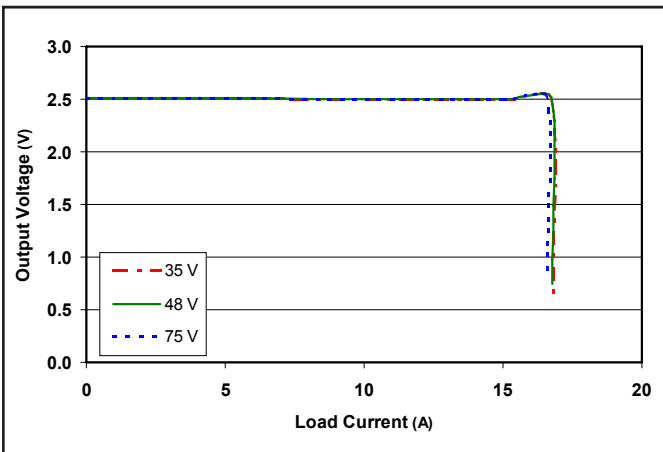
Figure 21: Output voltage vs. load current showing typical current limit curves and converter shutdown points for the 2.5\text{V} output. 3.3\text{V} load is at 0\text{A} .
