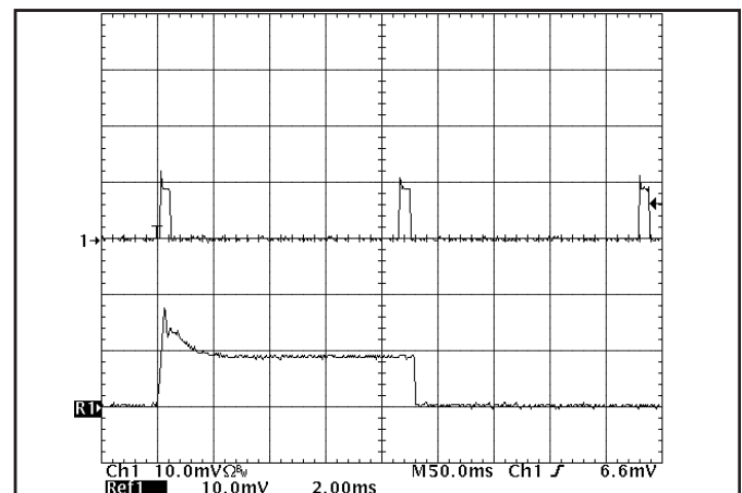
Figure 24: Load current for 3.3\text{V} output ( 20\text{A}/\text{div} ) as a function of time when the converter attempts to turn on into a 10\ \text{m}\Omega short circuit. Bottom trace is an expansion of the on-time portion of the top trace.
