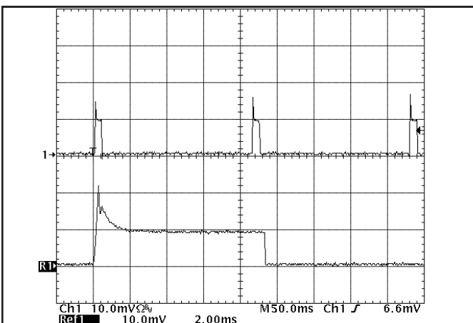
Figure 23: Load current for 2.5\text{V} output ( 20\text{A}/\text{div} ) as a function of time when the converter attempts to turn on into a 10\ \text{m}\Omega short circuit. Bottom trace is an expansion of the on-time portion of the top trace.
