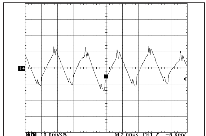
Figure 18: Input Terminal Ripple Current, 2.5V & 3.3V outputs at full rated output current and nominal input voltage with 10 \mu H source impedance and 100 \mu F electrolytic capacitor (10 mA/div). (see Fig. 17)
