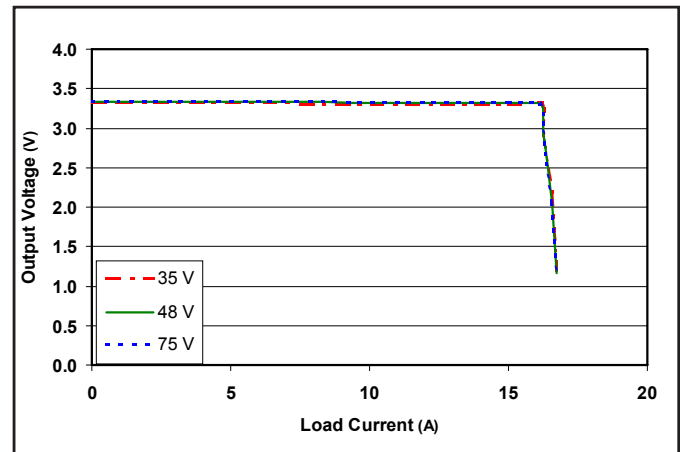
Figure 22: Output voltage vs. load current showing typical current limit curves and converter shutdown points for the 3.3\text{V} output. 2.5\text{V} load is at 0\text{A} .
