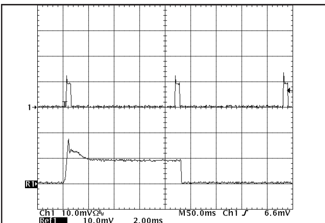
Figure 23: Load current for 1.8V output (20A/div) as a function of time when the converter attempts to turn on into a 10 m\Omega short circuit. Bottom trace is an expansion of the on-time portion of the top trace.
