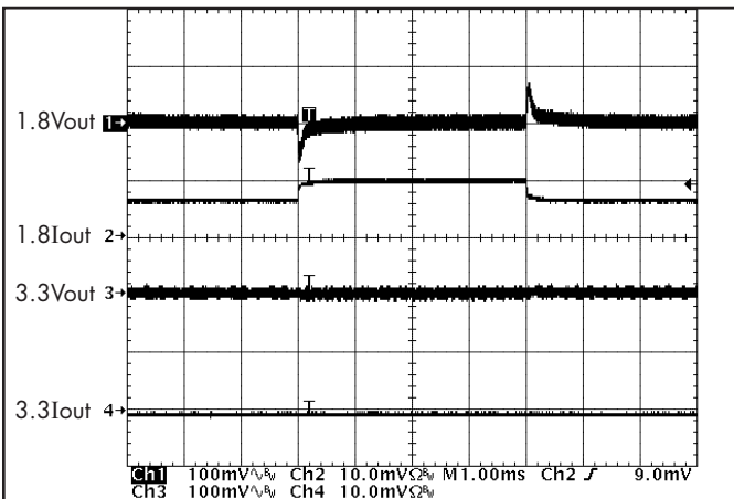
Figure 15: Output voltage response to step-change in I_{out1} (50%-75%-50% of I_{max} ; di/dt = 0.1A/\mu s ). Load cap: 15\mu F , 300\text{ m}\Omega ESR tantalum & 1\mu F ceramic. V_{out} (100mV/div), I_{out} (10A/div). Ch1: V_{out1} ; Ch2 I_{out1} ; Ch 3: V_{out2} ; Ch 4 I_{out2}
