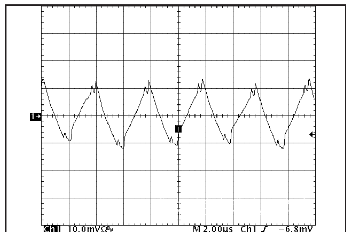
Figure 18: Input Terminal Ripple Current, 1.8V & 3.3V outputs at full rated output current and nominal input voltage with 10\mu H source impedance and 100\mu F electrolytic capacitor (10 mA/div). (see Fig. 17)
