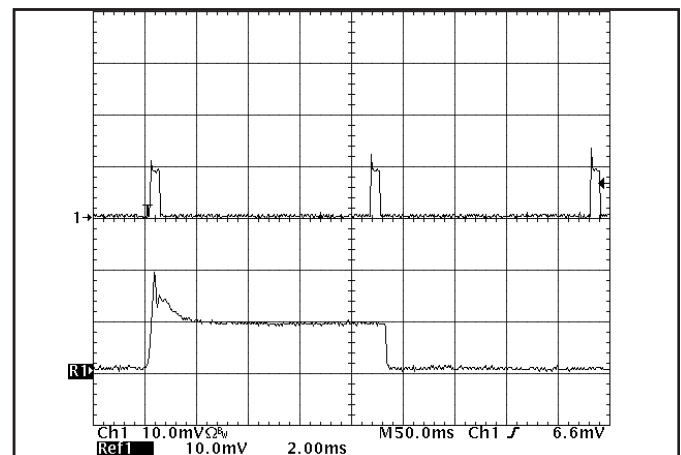
Figure 24: Load current for 3.3V output (20A/div) as a function of time when the converter attempts to turn on into a 10 m\Omega short circuit. Bottom trace is an expansion of the on-time portion of the top trace.
