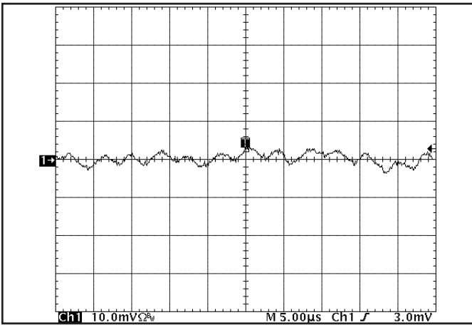
Figure 19: Input Reflected Ripple Current, i_s , through a 10 \mu H source inductor at nominal input voltage and rated load current (5 mA/div). 1.8V and 3.3V outputs at full rated load current. (see Fig. 17)
