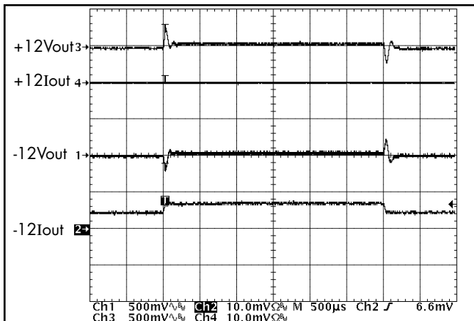
Figure 21: Output voltage response to step-change in Iout1 (50%-75%-50% of Imax; dI/dt = 0.1A/μs). Load cap: 15μF, 300 mΩ ESR tantalum cap & 1μF ceramic cap. Vout (500mV/div), Iout (5A/div). Ch1: Vout1; Ch2 Iout1; Ch 3: Vout2; Ch 4 Iout2
