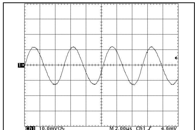
Figure 24: Input Terminal Ripple Current, -12V & +12V outputs at 50% rated output current and nominal input voltage with 10μH source impedance and 100μF electrolytic capacitor (200 mA/div). (see Fig. 23)
