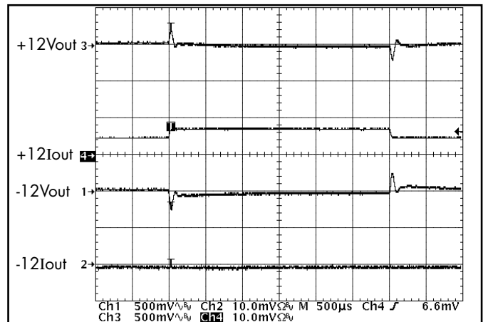
Figure 22: Output voltage response to step-change in Iout2 (50%-75%-50% of Imax; dI/dt = 0.1A/μs). Load cap: 15μF, 300 mΩ ESR tantalum cap & 1μF ceramic cap. Vout (500mV/div), Iout (5A/div). Ch1: Vout1; Ch2 Iout2; Ch 3: Vout2; Ch 4 Iout2
